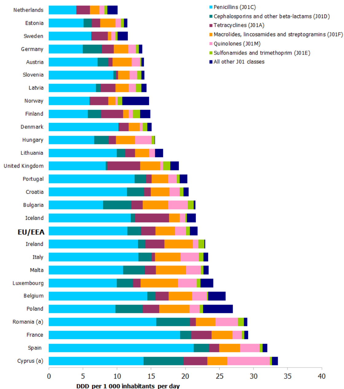
Figure 3. Consumption of antibacterials for systemic use (ATC group J01) by country and ATC group level 3 in the community, EU/EEA countries, 2017, expressed as DDD per 1 000 inhabitants per day
